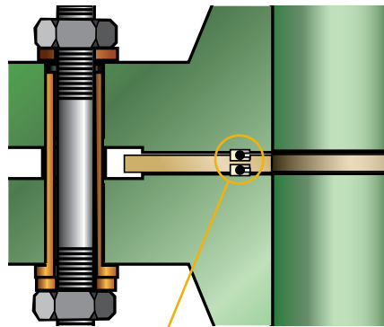
Spring PTFE Seals
